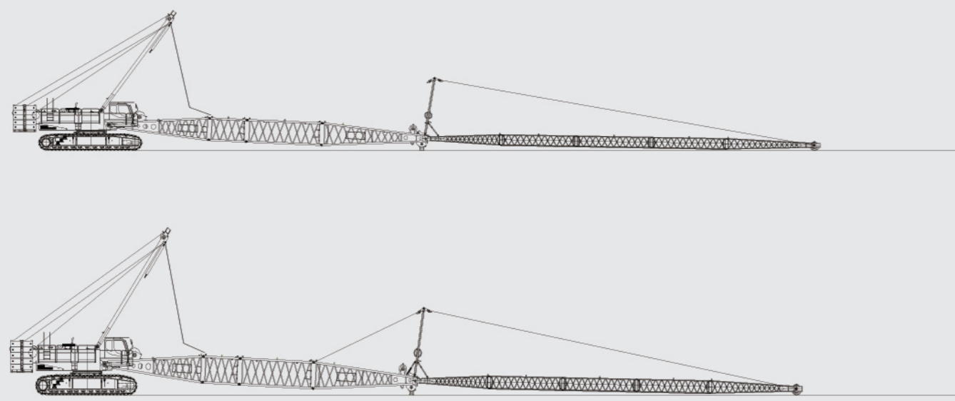
固定副臂安装示意图 Fixed Jib Installation Illustration
